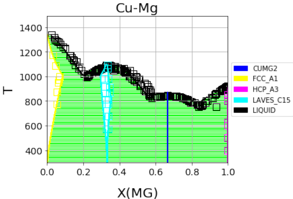
Fig. 4.2: Optimized Cu-Mg phase diagram from the multi-phase fitting in ESPEI
