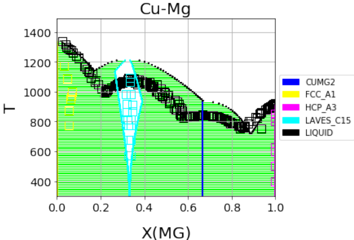
Fig. 4.1: First-principles Cu-Mg phase diagram from the single-phase fitting in ESPEI
