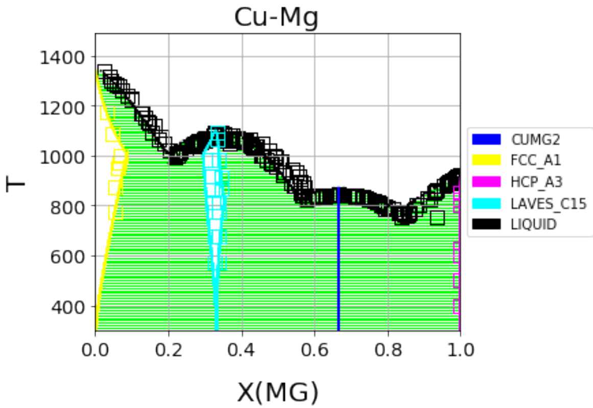
Fig. 5.2: Optimized Cu-Mg phase diagram from the multi-phase fitting in ESPEI
